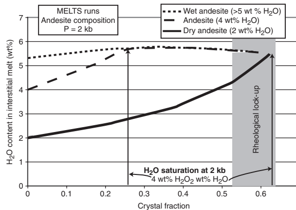
Fig. 3. Curves obtained by MELTS (Version 5.0, Ghiorsio & Sack, 1995) of crystal fraction vs H_2O content in interstitial melts for an andesite composition crystallizing at 2 kb pressure for different initial H_2O contents, illustrating the delayed water saturation in drier system, leading to a reduced eruptability.
